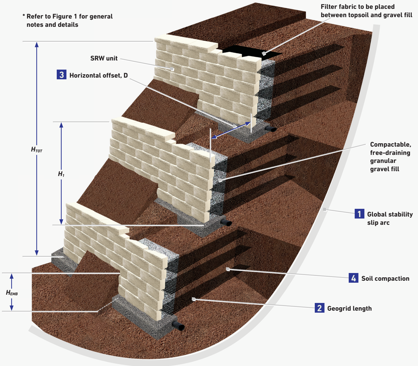
Figure 10 | Terraced Walls
