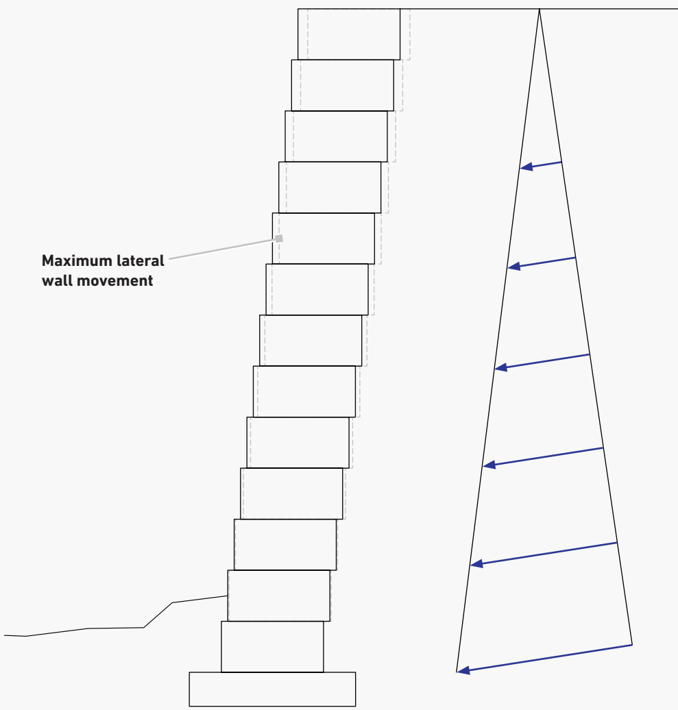
Figure 14.4 | Wall Section
