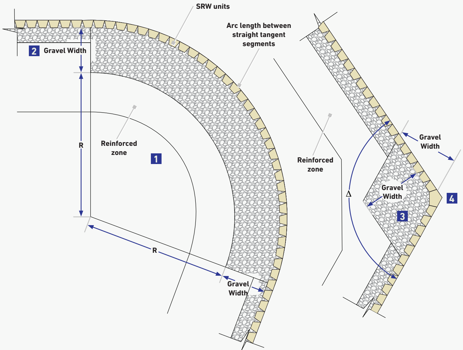
Figure 14 | Gravel Width Placement on Curves and Corners
