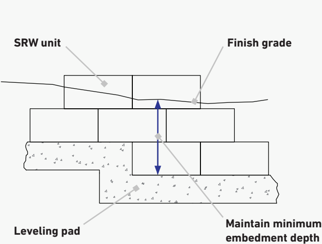
Figure 5.8-1 | Wall Step-Ups
