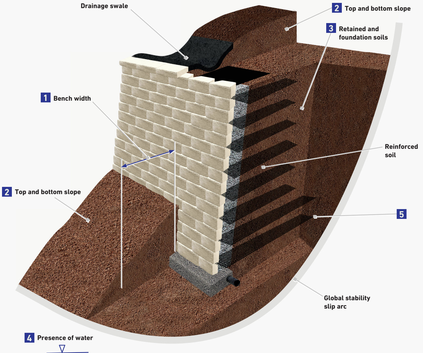
Figure 9 | Global Stability
