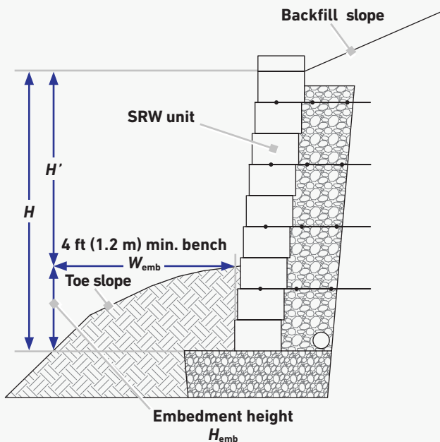
Figure 1.3-1 | Minimum Wall Embedment Depth, H_{emb}
