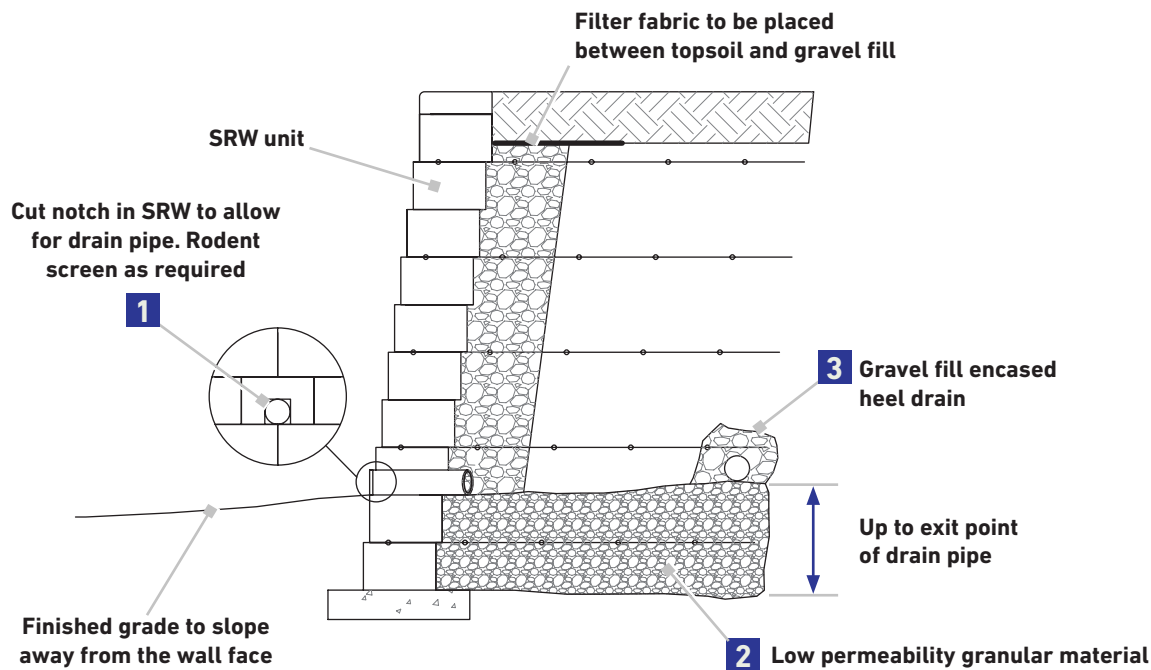
Figure 4.1.2-9 | Alternate Drain Pipe Detail
