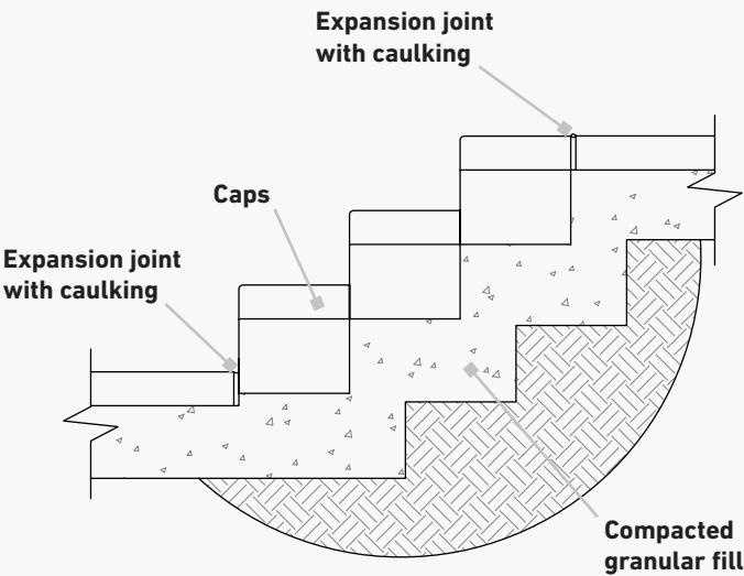
Figure 5.9-1 | Stair Construction
