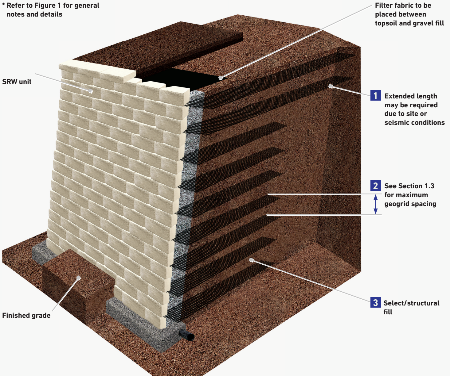
Figure 12 | Seismic Considerations
