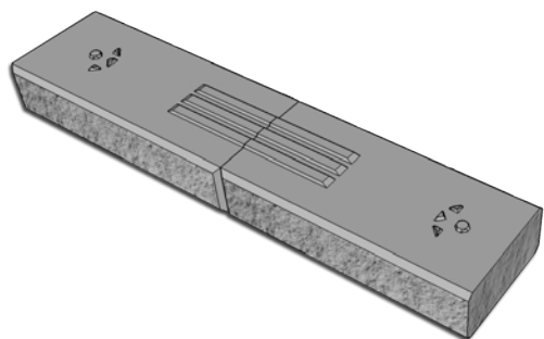
Ridge-to-Ridge &amp; Key-to-Key Installation (Best Practice where possible)
