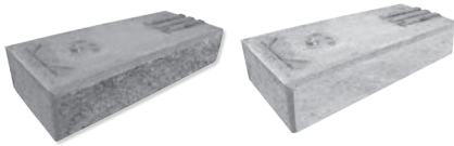
435 SPLIT BLOCK* / 435 SMOOTH BLOCK 39.4w x 7.68h x 17.1d in 1000w x 195h x 435d mm
