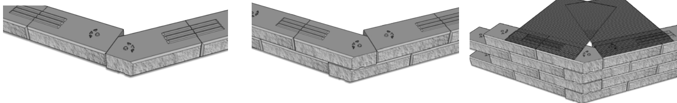
45 Corner - Row 1 &amp; 2 (Continue same sequence for following rows) + typical grid placement
